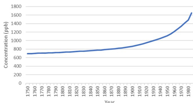
Figure 6a. Global Atmospheric Concentration of Methane (1750-1985)
